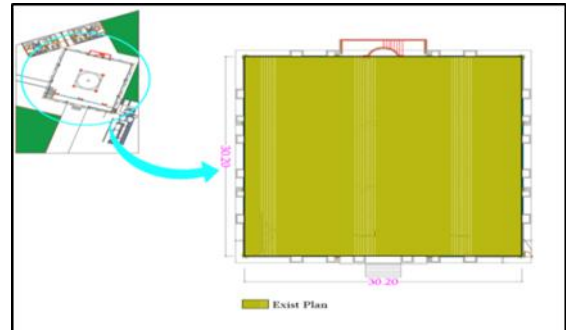
Figure 11. The actual dimensions of the prayer hall in Madina Mnawara Mosque (authors).
