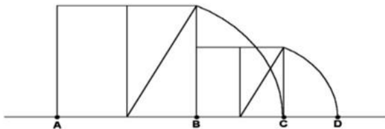
Figure 3. Construction of the golden section by extension [12].
