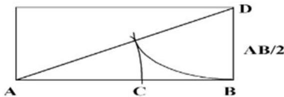
Figure 2. Construction of the golden section by division [1] [10]
