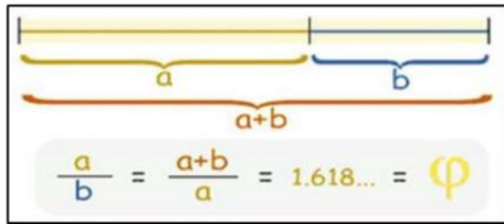
Figure 1. Golden Ratio through line segment [1].
