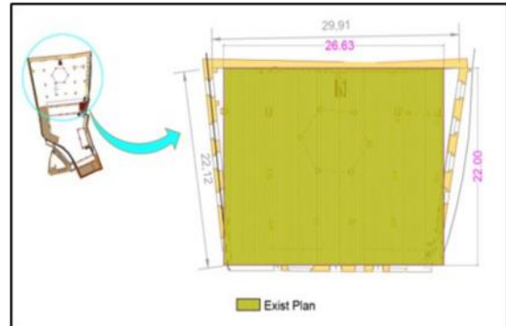
Figure 7. The actual dimensions of the prayer hall in the great mosque of Erbil Citadel (authors).
