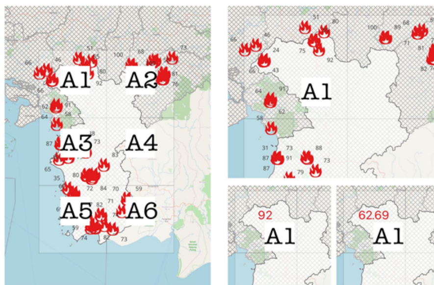
Figure 4: The illustration of the confidence levels of hotspots over six grids
