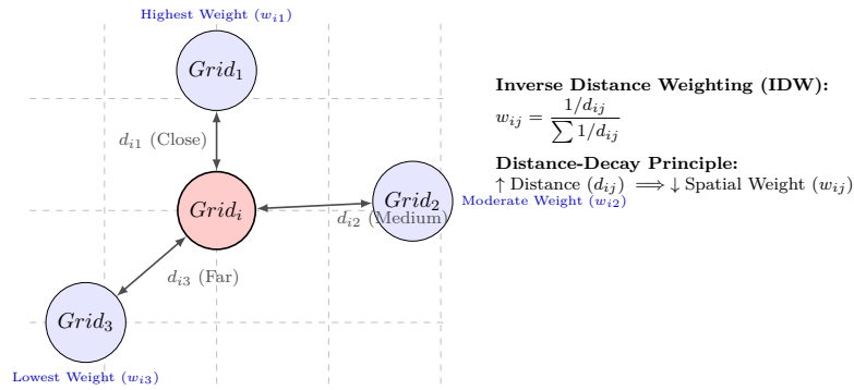
Fig. 2: Conceptual illustration of the standard Inverse Distance Weighting (IDW) spatial interaction structure among regular grid centroids based on the distance-decay principle.
