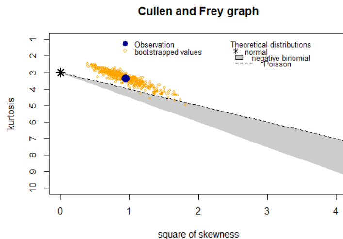
Fig. 2: Cullen and Frey Graph of the Number of Tuberculosis Cases used in the Study
