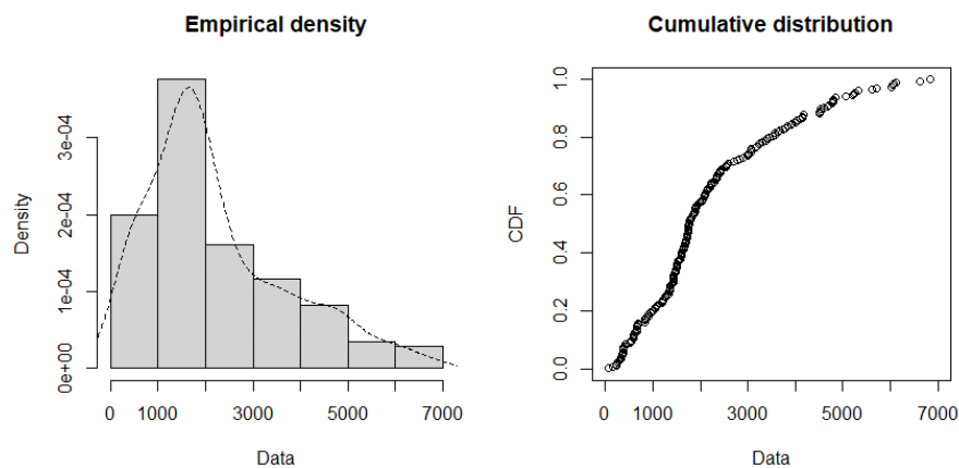
Fig. 1: Histogram and CDF of the Number of Tuberculosis Cases
