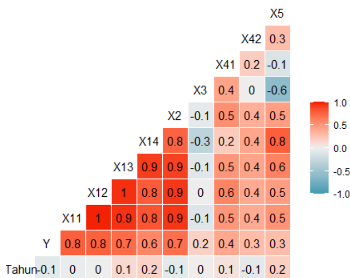
Fig. 3: Correlation between the variables of this study
