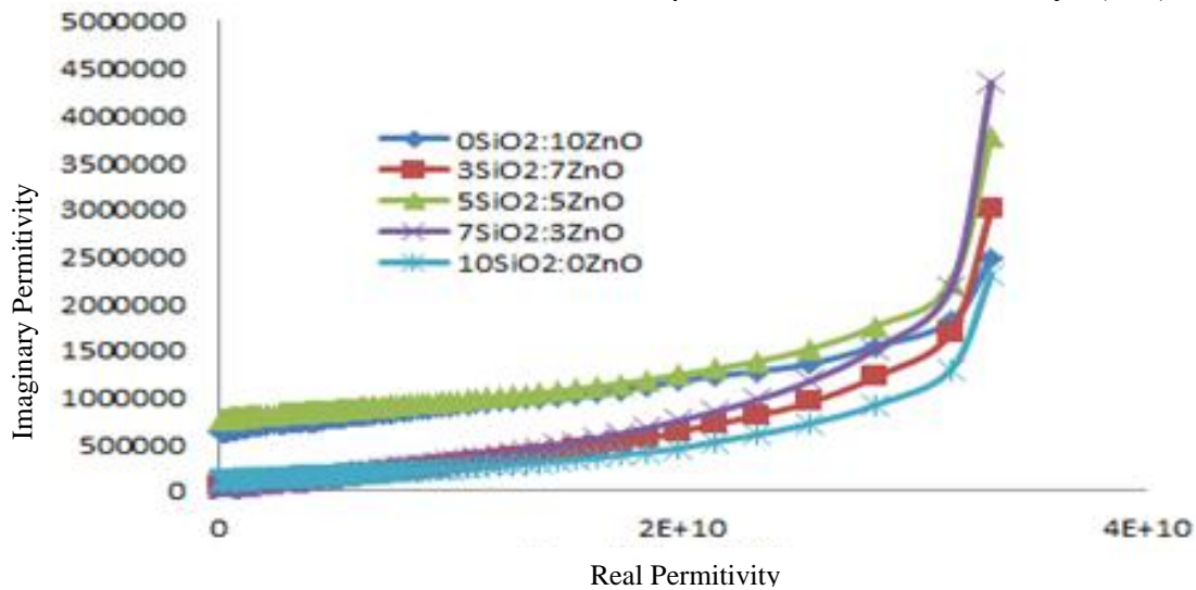
Figure 5. The relation between real permittivity and imaginary permittivity of samples
