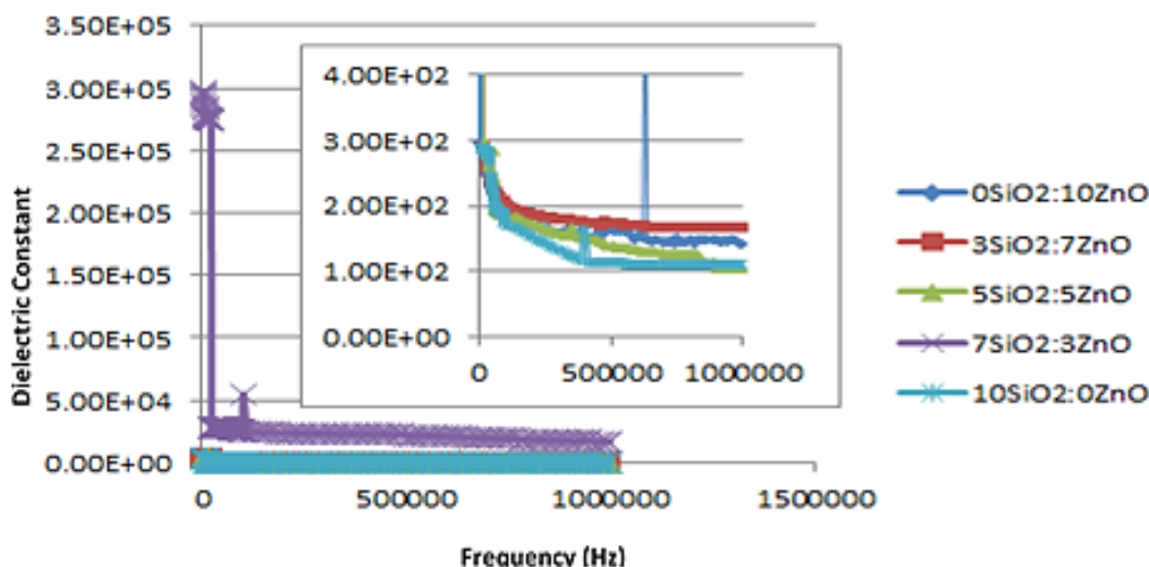
Figure 2. Frequency influence towards dielectric constant for the SiO 2 -ZnO nanocomposite
