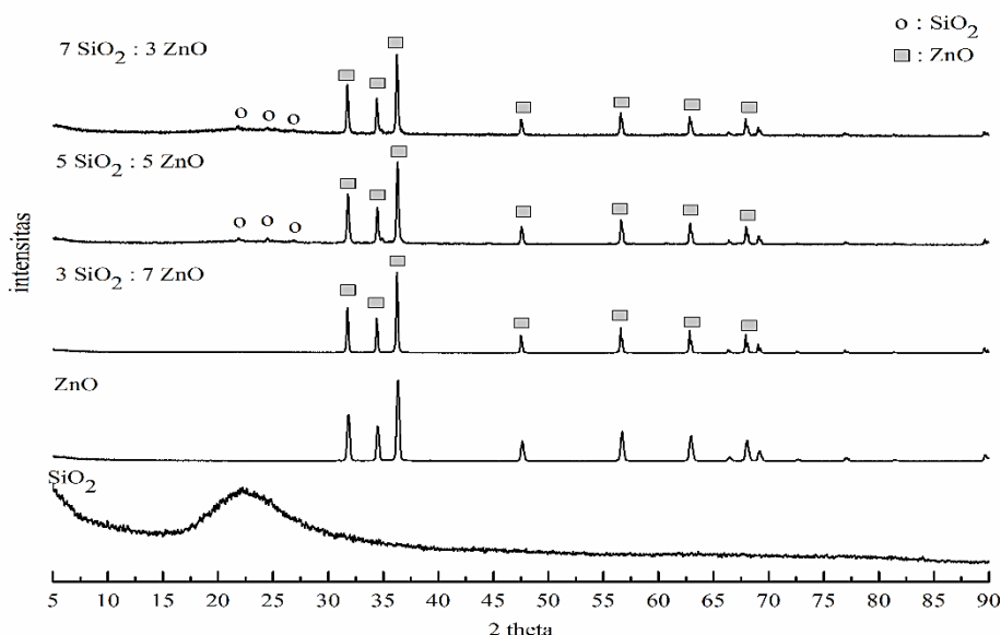
Figure 1. XRD graph of the \text{SiO}_2 : ZnO nanocomposite at a calcination temperature 600^\circ\text{C} with different composition mixings
