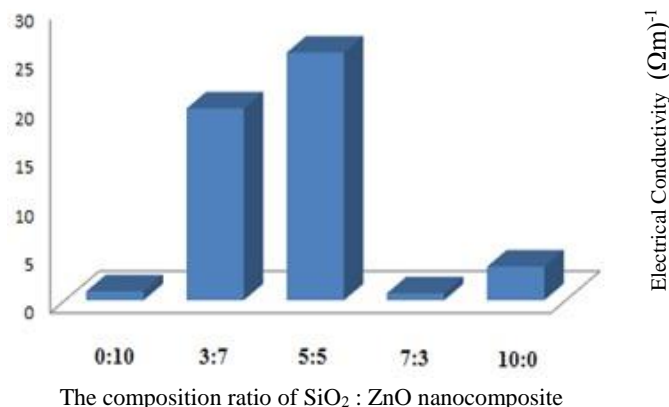
Figure 6. The relation between the composition ratio of SiO 2 : ZnO to electrical conductivity
