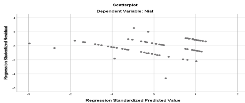
Figure 3. Graph of Heteroscedasticity Test Plot
